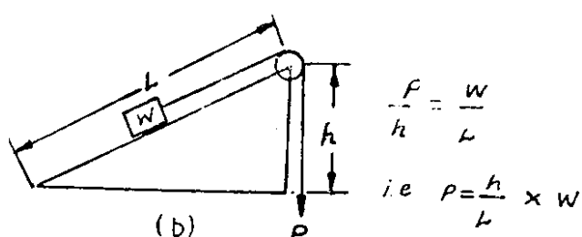
Fig. 3 : Stevin’s Law of Equilibrium Forces on an Inclined plane.
